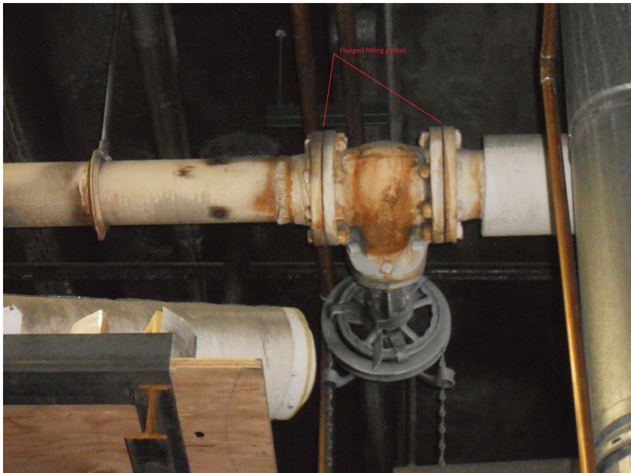
Example of flanged fitting gaskets.
